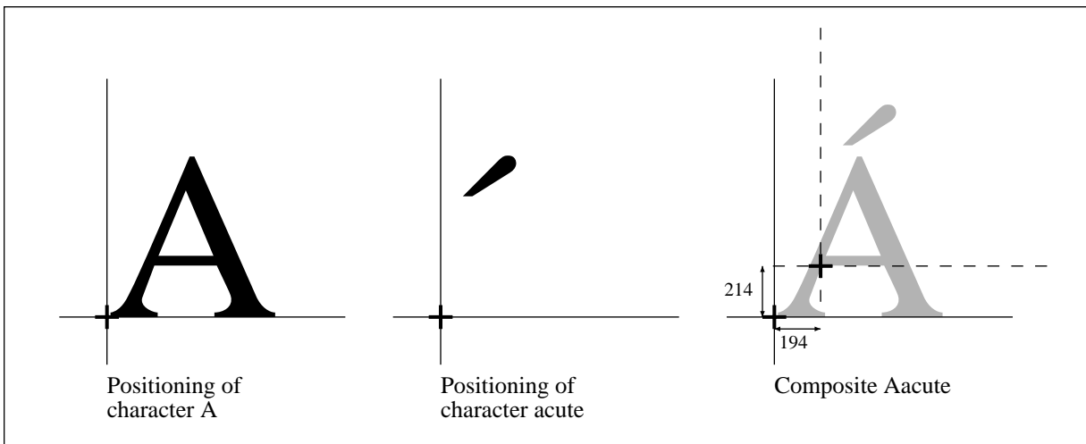
Figure 4 Positioning for a composite character
