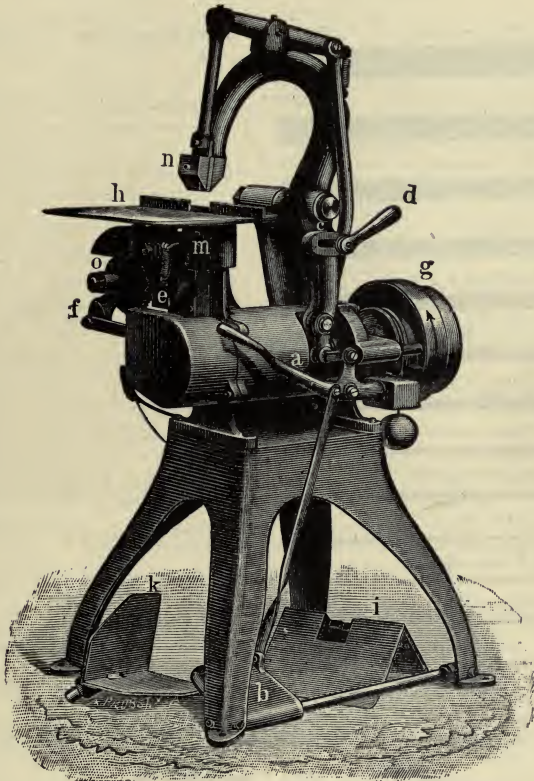
THE SUCCESS—NO. 7½—FOR STEAM POWER.
