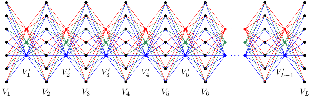
Figure 4: The graph H in the proof of Theorem 21.
