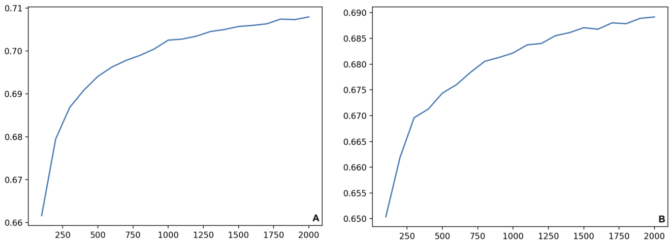
FIG. 1. Energy plots for two variants of the local greedy algorithm for finding a local optimum. The x axis in each plot is the value of the dimension n which takes values n = 100, 200, 300, \dots, 2000 . The y axis is the value of H(\sigma)n^{-3/2} when the algorithm halts, averaged over 100 runs of the algorithm. The algorithm used in (a) is the local greedy rule whereby the first coordinate that gives an improvement in energy is flipped at each step. In (b), the coordinate giving the largest improvement is used at each step.
