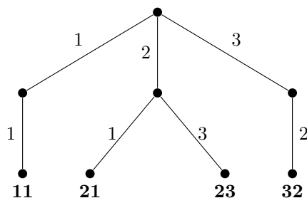
FIG. 1. An example of a trie with alphabet \{1, 2, 3\} .
