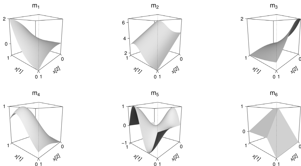
Fig. 1. Behavior of the test functions m_1, m_2, m_3, m_4, m_5, m_6 .
