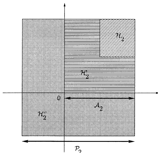
Fig. 1. Examples of sets \mathcal{P}_2 , \mathcal{A}_2 , \mathcal{H}_2 , \mathcal{H}'_2 and \mathcal{H}''_2 .
