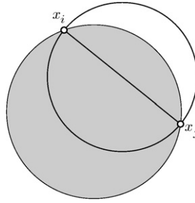
Fig. 3. If (x_i, x_j) is a Delaunay edge, then one of two halfcircles supported by (x_i, x_j) must be empty.
