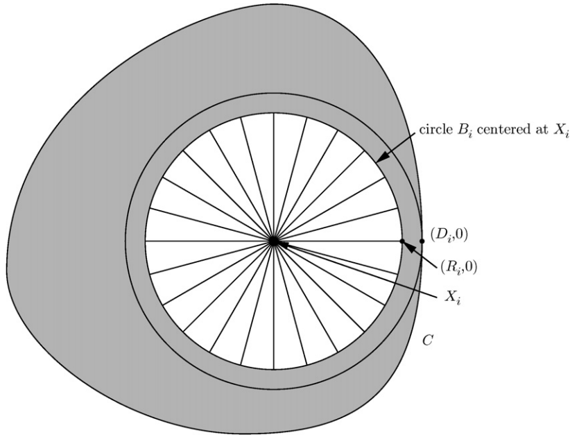
Fig. 2. The convex region C is shaded. A point X_i is a border point if one of the 24 cones centered at it, of radius R_i = D_i\sqrt{3}/2 , contains no other data point. Here D_i is the distance from X_i to the complement of C .
