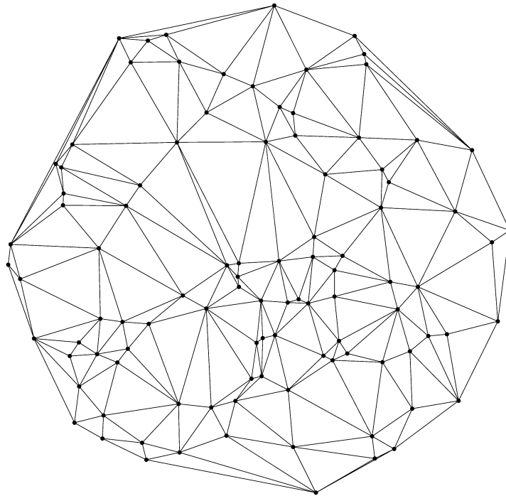
Fig. 1. A point set with its Delaunay triangulation. No circle circumscribing any triangle has any data point in its interior.
