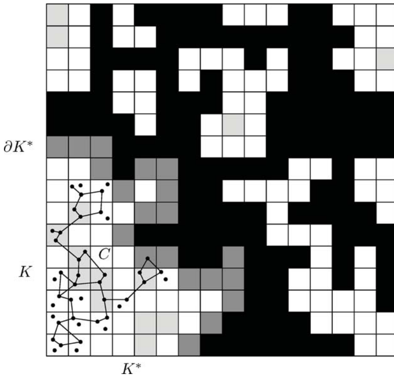
Fig. 2. The component C with its corresponding * -connected component of occupied cells K . We enlarge K by adding all the connected white and gray cells to get K^* . The border cells of K^* are colored in dark gray.
