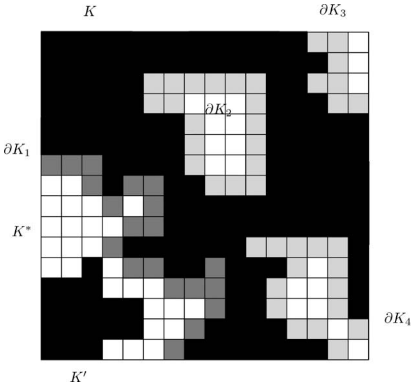
Fig. 1. The two components K and K' separated by the * -connected piece of the boundary \partial K_1 . The boundary of K is colored in gray and \partial K_1 in dark gray. The boundary of K'' is \partial K_1 .
