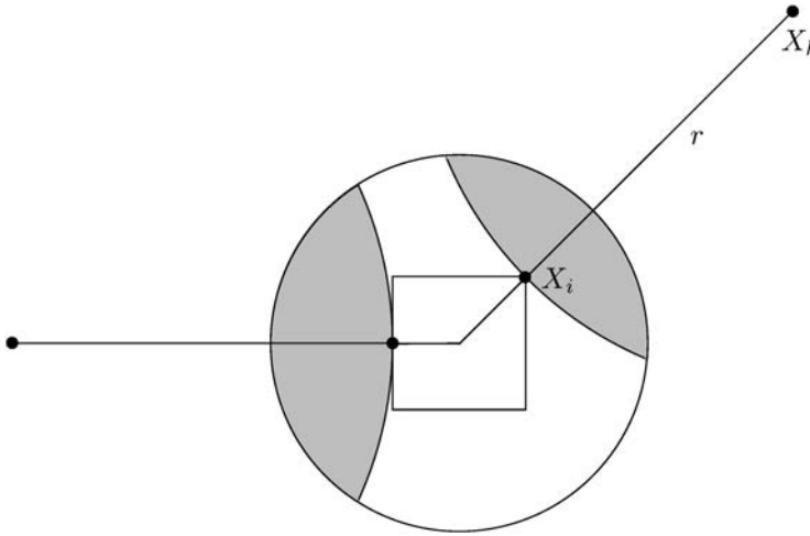
Fig. 3. For any point X_i in a box of edge length \ell , if h \in N_i is a neighbor selected by i , then h may select neighbors within distance r/2 of the center of the square from the shaded regions—the so-called “moons”. The volume of any moon is at least a constant times r^d . The figure shows two possible positions of X_i in a box with a corresponding neighbor and moon.
