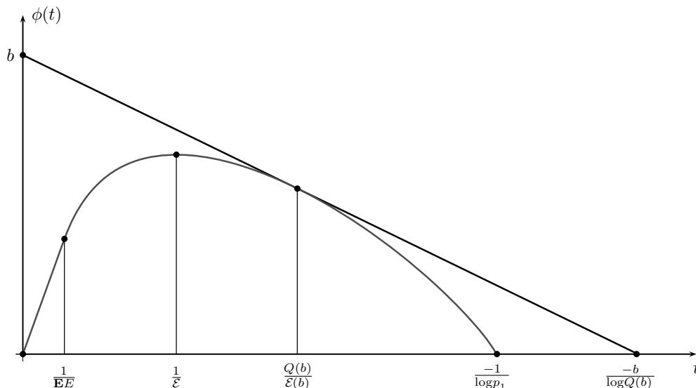
Figure 7. The diagram explaining the profile of the core (concave curve) and the behaviour of the spaghetti (straight line) for the case of ordinary tries.
