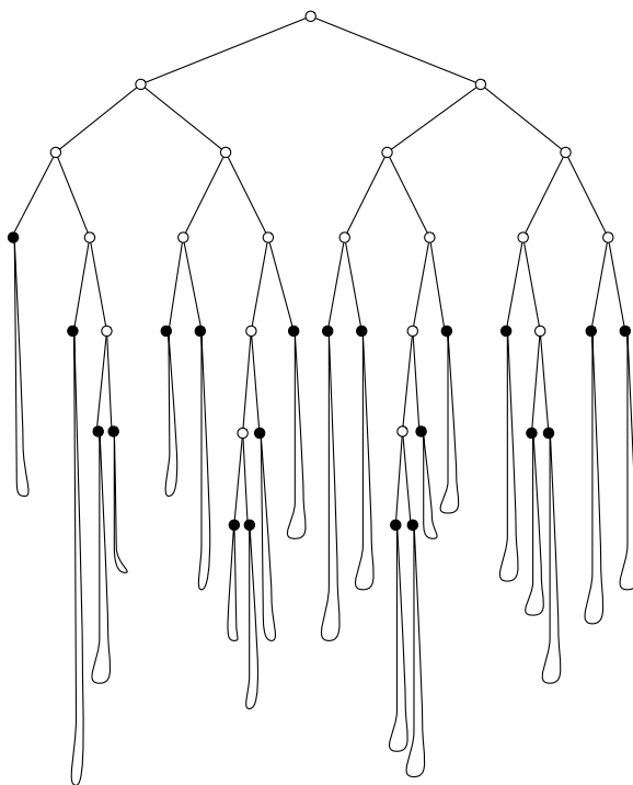
Figure 1. The structure of a trie: the bulk is the core; then some spaghetti-like trees hang down from the core. Both the core and the spaghettis contribute significantly to the height of the trie. Observe also that the height may not be explained by a spaghetti born at one of the deepest nodes of the core. This latter fact will become clear later.
