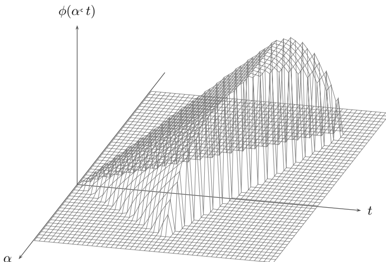
Figure 9. The weighted profile of the core for the question of path imbalance for p = 0.3 . When looking at levels deep in the core, the nodes have mostly negative imbalance due to the fact that p < 1/2 .
