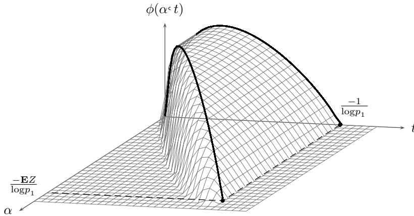
Figure 3. A typical logarithmic profile 0 \vee \phi(\alpha, t) . The thick black lines represent \phi(0, t) and \phi(tEZ, t) . For t_0 constant, \phi(\alpha, t_0) is constant for \alpha \in [0, t_0EZ] .
