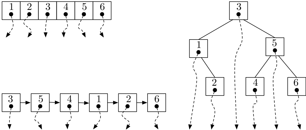
Figure 8. The different node structures used for the standard (top left), list (bottom left) and bst-trie (right) when the order of appearance of the characters is 3, 5, 4, 1, 2 and 6. The dashed arrows represent the pointers to further levels of the trie.
