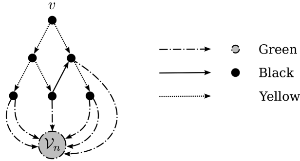
Fig. 4. An example of \mathcal{T}_v .
