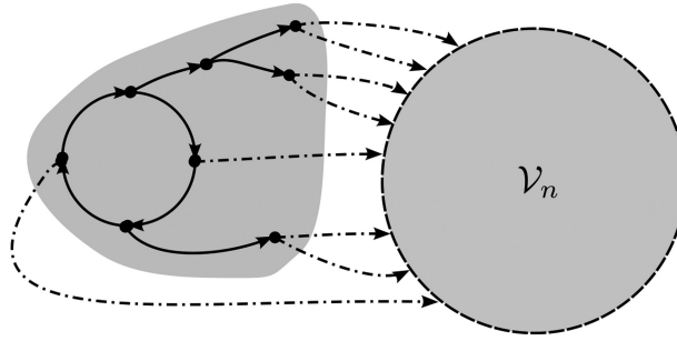
Fig. 3. The leftmost shaded part of this figure is an \ell -eye.
