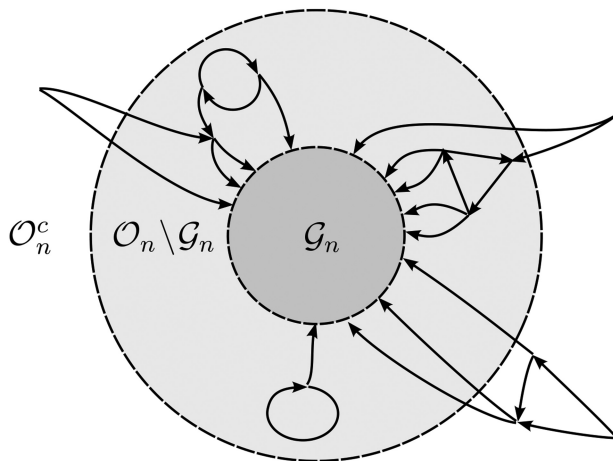
Fig. 1. Three layers of \mathcal{D}_{n,k} : the giant \mathcal{G}_n ; the one-in-core \mathcal{O}_n ; and the whole graph.
