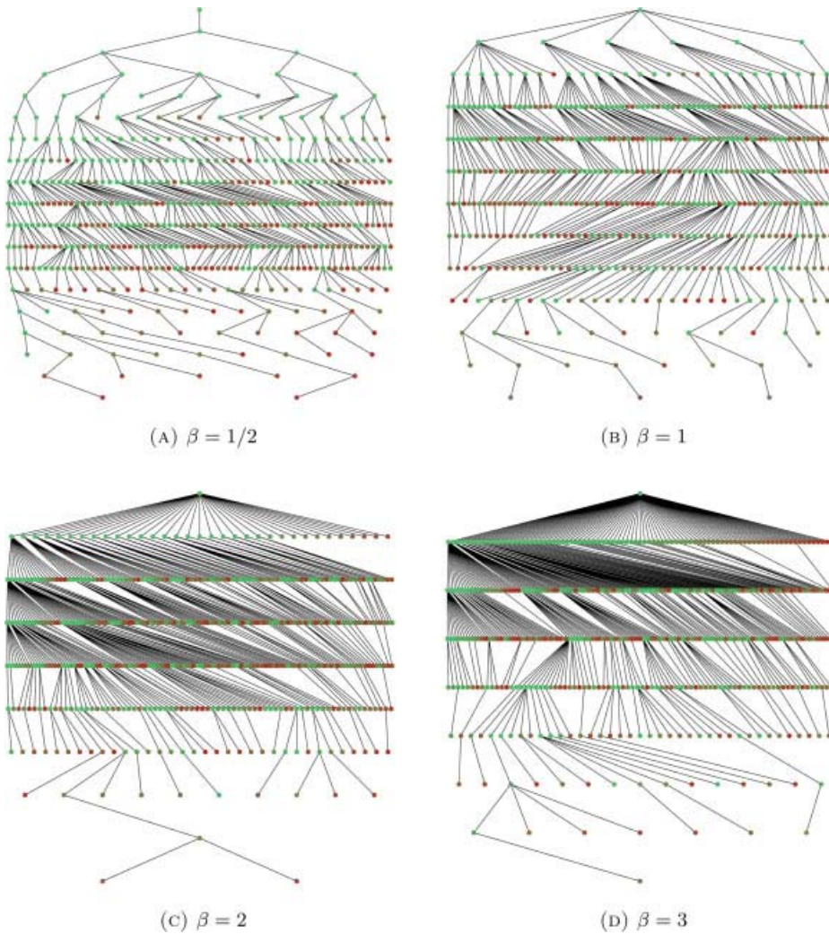
Fig. A1. SARRT with distribution U^\beta and n = 500 . [Color figure can be viewed in the online issue, which is available at wileyonlinelibrary.com .]
