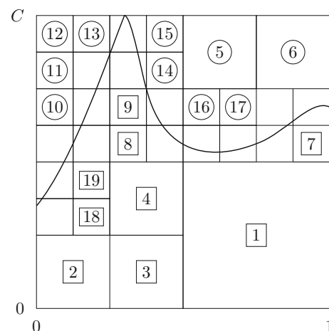
Fig. 1 Decomposition of [0, 1] \times [0, C] into its quadtree tree structure
