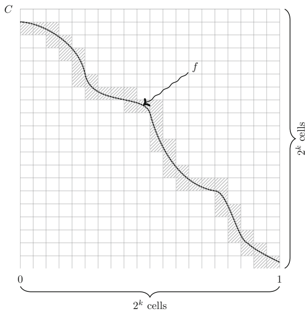
Fig. 3 The number of cells visited by the monotone curve f is at most 2 \cdot 2^k cells
