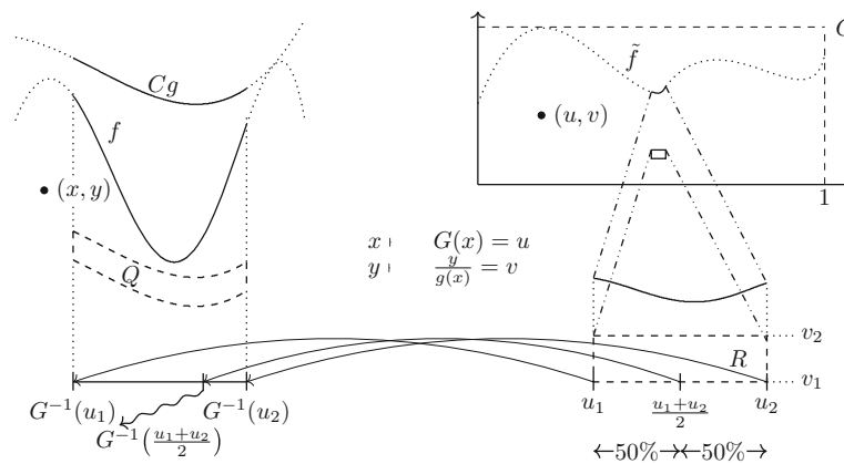
Fig. 4 An accepting uniform random rectangle R and the bisection of its back-transformation Q : (u, v) \in R if and only if (x, y) \in Q
