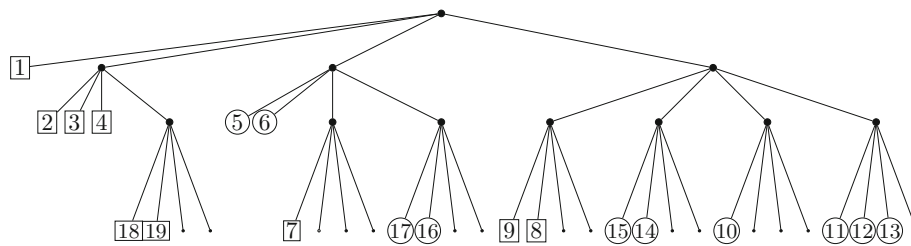
Fig. 2 Quadtree for decomposition on Fig. 1
