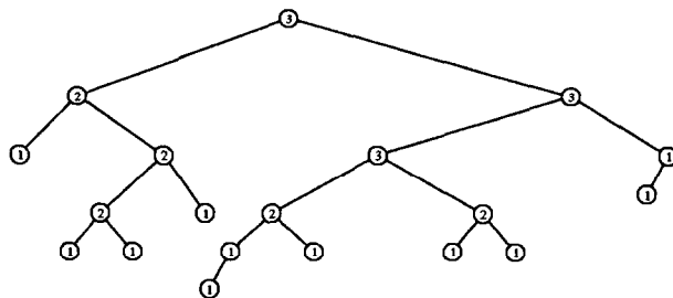
Fig. 1. A binary tree with Horton–Strahler number three.
