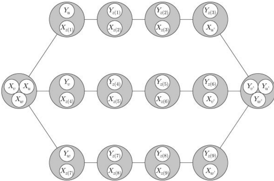
Fig. 5. The multigraph for the r -worm when r = 4 . The leftmost occurrence of a datum such as u is for the first string of that datum ( X_u ), while the rightmost occurrence is for the second string ( Y_u ).
