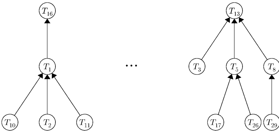
Fig. 4. The forest G is maintained by organizing each tree component in a parentpointer tree. The components in the figure might correspond, for example, to the list of strings given in the previous figure.
