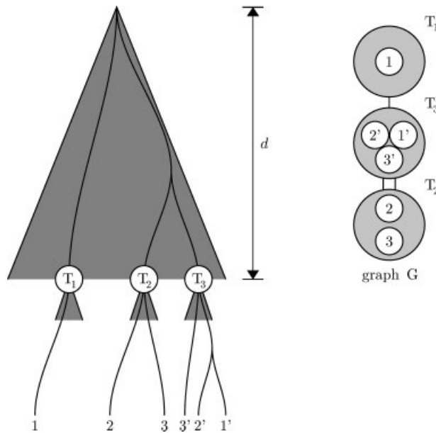
Fig. 2. The multigraph G and an infinite trie for n = 3 pairs of strings, denoted by (1, 1') , (2, 2') and (3, 3') . Note that (2, 2') and (3, 3') is a colliding pair.
