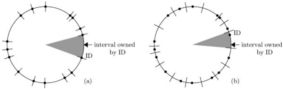
Fig. 1. Two ways of partitioning the space. In both (a) and (b), IDs are randomly generated on the perimeter. In (a), IDs own the intervals to their left in clockwise order. In (b), IDs own an interval whose boundaries are determined in some manner, e.g., by virtue of a trie or digital search tree. A downloader or user generates a random number X on the perimeter and picks the owner of the interval of X for its job. The objective is to make all intervals of about equal length, so that all hosts receive about equal traffic.
