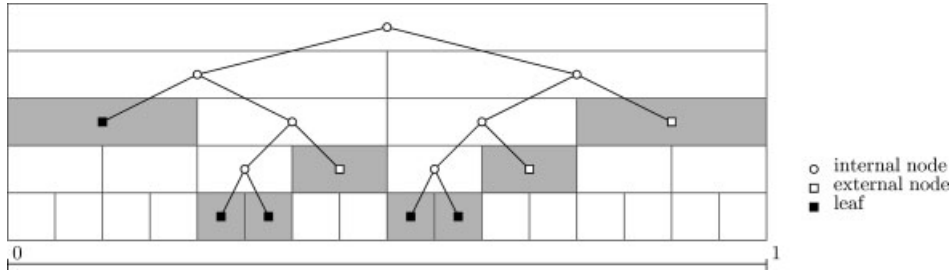
Fig. 6. A standard trie for five strings. The correspondence between nodes and intervals in a dyadic partition of the unit interval is shown. The leaf ID assigned is read from the path to the root (0 for left, 1 for right). The external nodes, not normally part of the trie, are shown as well. Together, external nodes and leaves define a partition of the unit interval (shaded boxes). The fill-up level of this tree is one, while the height is four.
