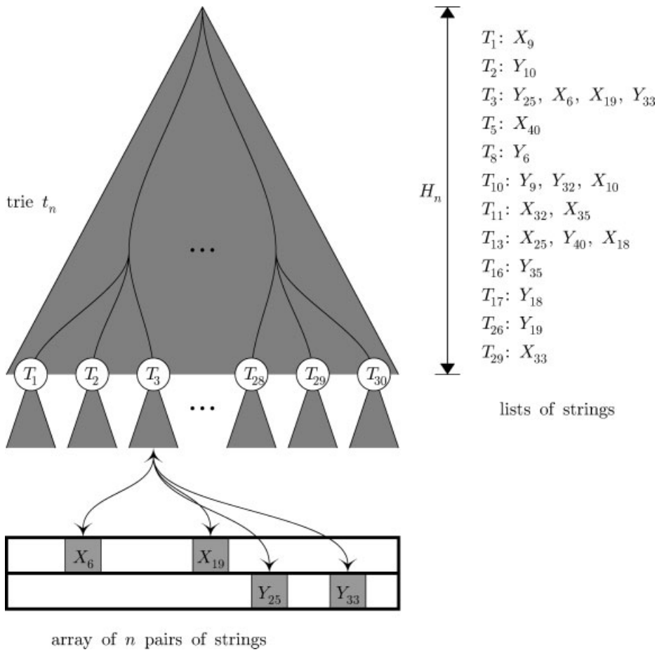
Fig. 3. The basic data structure needed to efficiently construct the two-choice trie in an online manner.
