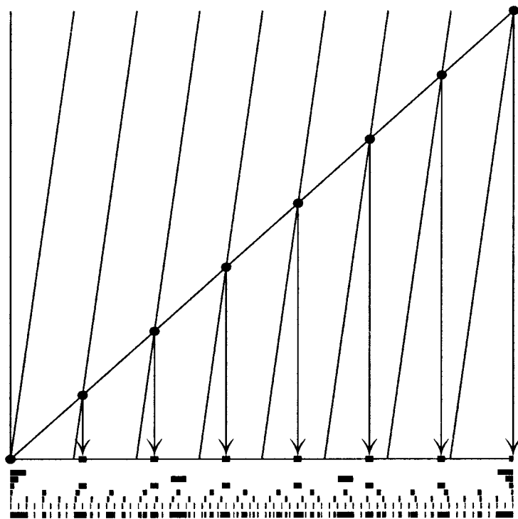
Fig. 2. The last line shows the bad set B_n(\xi) for m = 6 and \xi = 3/50 . The six lines above show the sets \{|x - T^k(x)| \leq \xi\} for k = 1, \dots, 6 . In the square, for the case k = 3 , it is shown how these sets emerge.
