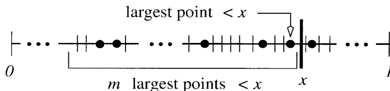
Fig. 3. The interval [0, 1] is shown with the m largest of the points Z_1, \dots, Z_{i+m-1} less than x , where the lines mark those of these m points belonging to \{Z_1, \dots, Z_i\} and the dots mark the corresponding points from \{Z_{i+1}, \dots, Z_{i+m-1}\} .
