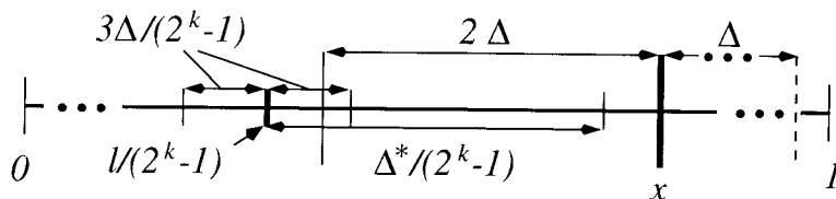
Fig. 4. Shown is a case, where the part \{|T^k(x) - x| < 3\Delta\} of the bad set B_n(3\Delta) intersects the interval [x - 2\Delta, x + \Delta] , while x is outside the part \{|T^k(x) - x| < \Delta^*\} of the bad set B_n(\Delta^*) .
