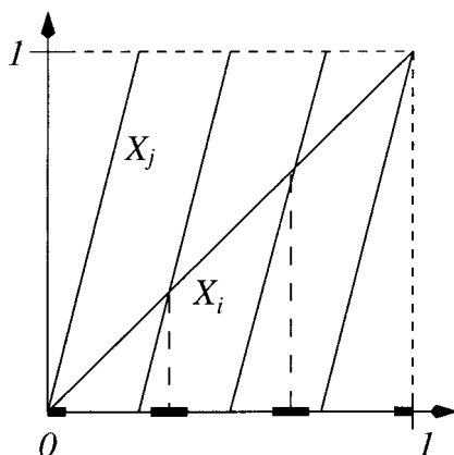
Fig. 1. Shown is the set \{|X_i - X_j| \leq \varepsilon\} for k = j - i = 2 and \varepsilon = 3/20 together with X_i and X_j , where X_i is modeled as the identity on [0, 1] .
