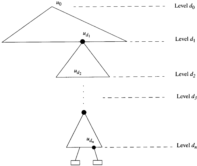
Fig. 2. The depths of the nodes on the path of X_{n+1} at which compaction takes place are denoted by d_0 = 0 < d_1 < d_2 < \dots .
