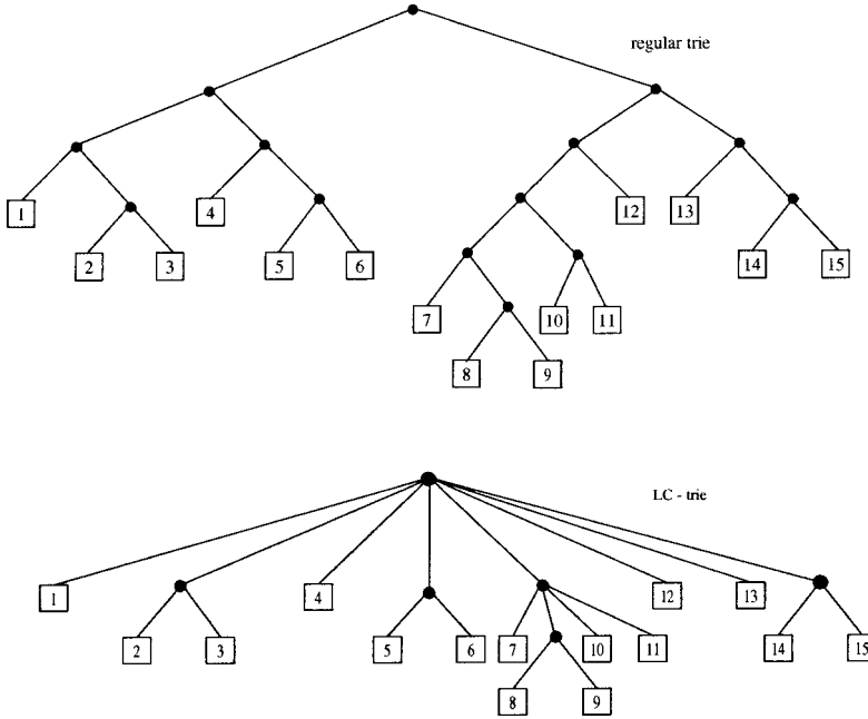
Fig. 1. A standard binary trie and the corresponding LC trie.
