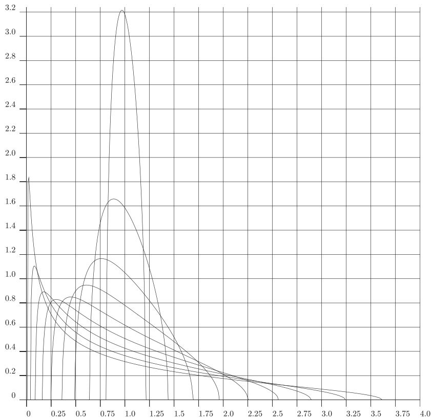
Fig. 1. Marchenko–Pastur densities for \sigma equal to 0.1, 0.2, 0.3, 0.4, 0.5, 0.6, 0.7, 0.8 and 0.9, from right to left.
