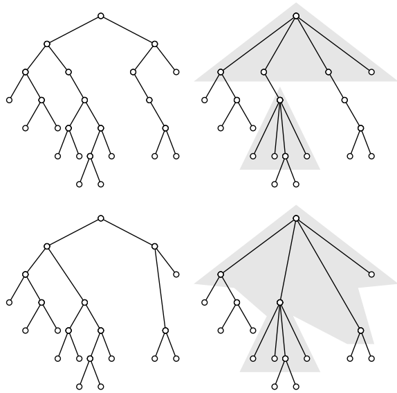
Fig. 1. At the top, from left to right: a binary trie, and the corresponding LC trie. At the bottom, left to right: the PATRICIA trie, and the LC PATRICIA trie obtained by level compaction from the PATRICIA trie. The compacted parts in the LC trie are highlighted.
