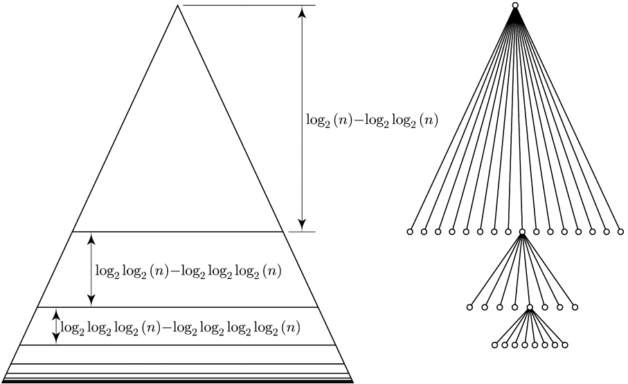
Fig. 2. The left figure shows the top \log_2 n levels of a random trie. Roughly speaking, such tries get compacted to LC tries (on the right) in the manner shown, with only minor random variations. The trie on the left has about \log^*(n) horizontal sections of nodes, each section corresponding to one level in the random LC trie. Therefore, most nodes in the LC trie are at a distance of about \log^*(n) from the root. However, the random fluctuations are such that the height of the LC trie is actually much larger.
