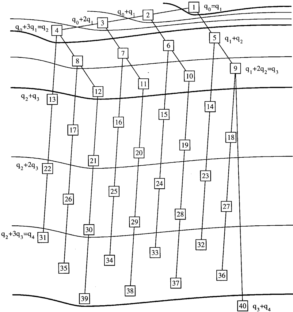
Fig. 1. This figure shows the Weyl tree for \theta = \sqrt{77} = [8; 1, 3, 2, 3, \dots] . Note that q_0 = 1 , q_1 = 1 , q_2 = 4 , q_3 = 9 , q_4 = 31 . Layers are separated by wiggly lines. Thicker lines separate layers of different polarity. Note that there are first a_1 layers of right polarity, followed by a_2 layers of left polarity, and so forth. Also note that just before an extremum, all leaves may be found in the last layer. The x -coordinates of the points are geometrically exact, to facilitate interpretation. Using Lemma 1, can the reader guess who the parent is of point 41?
