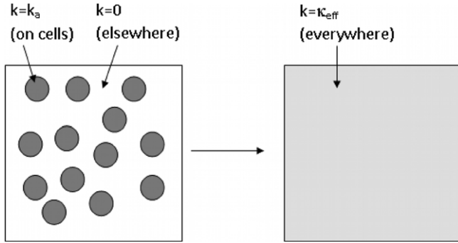
Fig. 2. Boundary homogenization procedure. As the receptors are present only on cell membranes, the surface rate constant k = k_a on cell surfaces (approximated by disks) and k = 0 elsewhere. In our simulations, we assume that the receptors are distributed uniformly on the whole surface. Therefore, the rate constant of the surface can be estimated as k_{\text{eff}} .
