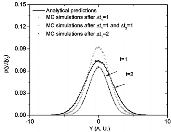
Fig. 6. Effect of the time steps on Q(t|x_0)p_y(y, t|y_0) for bound particles. For this simulation, k_1 = 1 , x_0 = 1 and L = 5 . The simulation is attempted with two time steps ( \Delta t_1 = 1 and \Delta t_2 = 1 ) and with one time step ( \Delta t_1 = 2 ). The distribution obtained with two time steps is different (see text for details).
