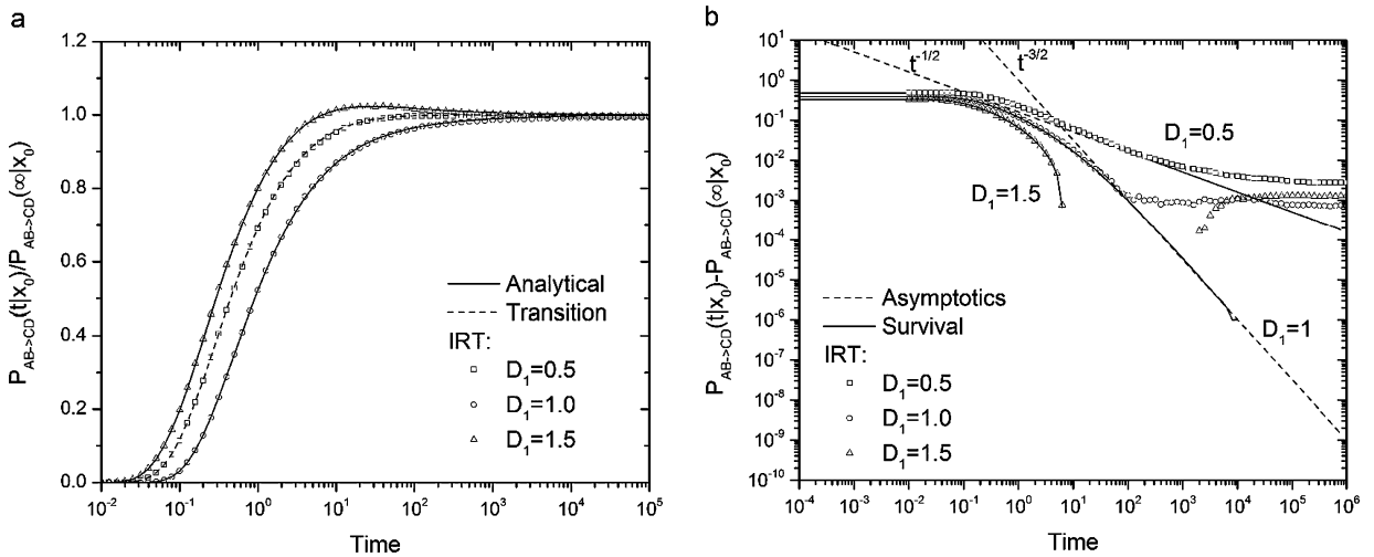
Fig. 3. Ratio P_{AB \rightarrow CD}(t|x_0)/P_{AB \rightarrow CD}(\infty|x_0) (a) and difference P_{AB \rightarrow CD}(t|x_0) - P_{AB \rightarrow CD}(\infty|x_0) (b) of the reaction probabilities for a pair initially in the state AB, with the parameters a_1 = 1 , k_1 = 5 , a_2 = 4 , D_2 = 1 , k_2 = 8 , x_0 = 1.625 , for D_1 = 0.5 , D_1 = 1.0 (transition) and D_1 = 1.5 . Simulations performed with the IRT methods (dots) are shown as well.
