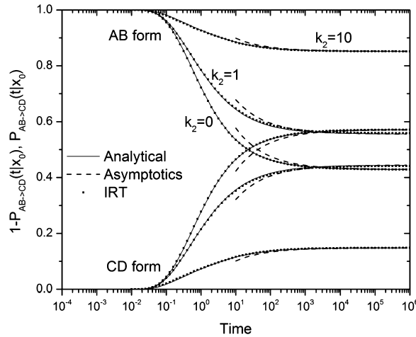
Fig. 2. Probability of the particles to be in the state AB (top) or CD (bottom), assuming that all particles are initially in the state AB at distance x_0 = 2.5 . The parameters are a_2 = 1 , D_1 = 1 , k_1 = 5 , a_2 = 1 , D_2 = 1 . The curves are plotted for k_2 = 0 , k_2 = 1 and k_2 = 10 . Analytical functions: (—); asymptotics: (---); results from IRT simulation: (■).
