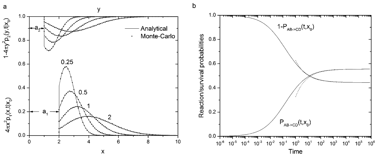
Fig. 1. (a) Green's functions 4\pi x^2 p_1(x, t | x_0) (bottom) and 1 - 4\pi y^2 p_2(y, t | x_0) (top) for x_0 = 2.5 , a_1 = 2 , D_1 = 1 , k_1 = 20\pi , a_2 = 1 , D_2 = 1 and k_2 = 4\pi , at 0.25, 0.5, 1 and 2 time units. Analytical functions: (—); result of sampling: (•). (b) Fraction of particles in the state AB ( 1 - P_{AB \rightarrow CD}(t, x_0) ) and in the state CD ( P_{AB \rightarrow CD}(t, x_0) ). The time is in arbitrary units.
